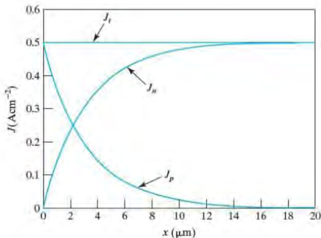
FIGURE III-1 Minority current density, majority current density, and the total current density.
