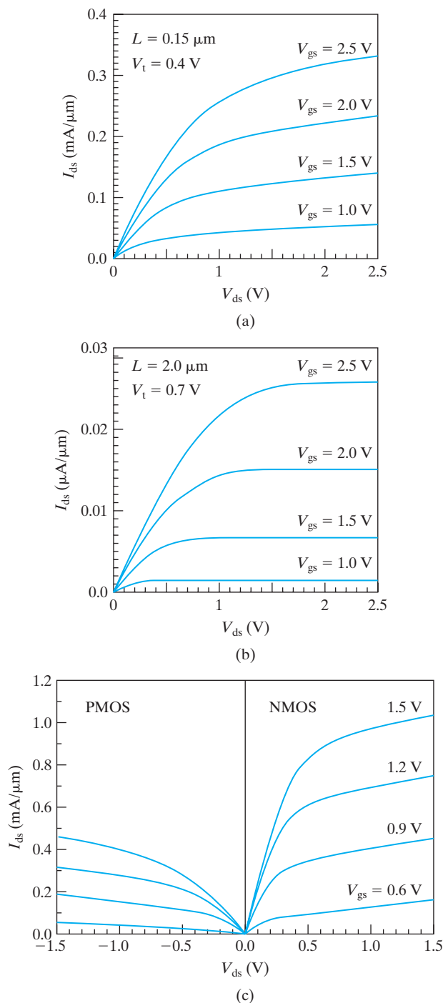
FIGURE 6-23 Measured IV characteristics. (a) A 0.15\ \mu\text{m} channel device ( V_t = 0.4\ \text{V} ) shows a linear relationship between I_{dsat} and V_{gs} . V_{dsat} is significantly less than V_{gs} - V_t . (b) A 2\ \mu\text{m} device ( V_t = 0.7\ \text{V} ) exhibits the I_{dsat} \propto (V_{gs} - V_t)^2 relationship. (c) IV characteristics of PFET and NFET with T_{oxe} = 3\ \text{nm} and L \approx 100\ \text{nm} .
