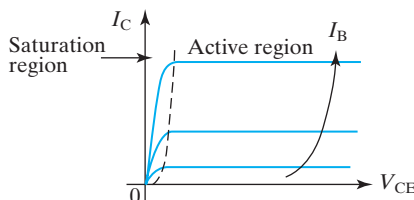
FIGURE 8–12 In the saturation region, I_C drops because the collector–base junction is significantly forward biased.
