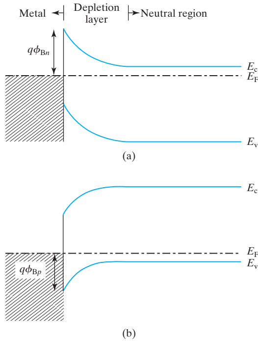
FIGURE 4–34 Energy band diagram of a metal–semiconductor contact. The Schottky barrier heights depend on the metal and semiconductor materials. (a) \phi_{Bn} is the barrier against electron flow between the metal and the N-type semiconductor; (b) \phi_{Bp} is the barrier against hole flow between the metal and the P-type semiconductor.
