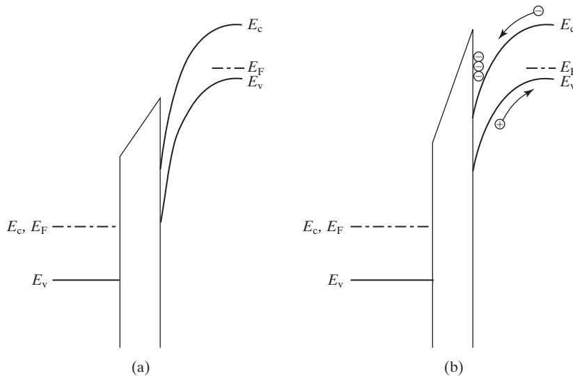
FIGURE 5–28 Deep depletion. (a) Immediately after a gate voltage V_g > V_t is applied, there are no electrons at the surface. (b) After exposure to light, photo-generated electrons have been collected at the surface. The number of electrons is proportional to the light intensity.
