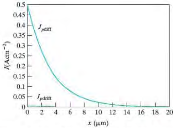
FIGURE III-2 The minority drift and diffusion currents. The drift current is negligibly small compared to the diffusion current.
