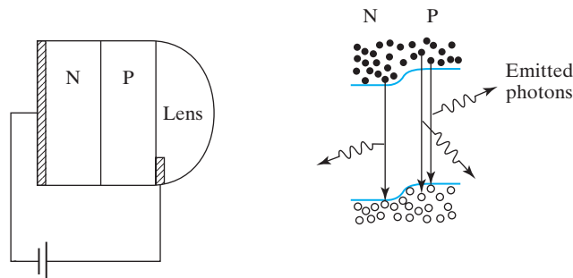
FIGURE 4–29 Schematic drawing of an LED. Photons are generated when the electrons and holes injected by the PN junction recombine.
