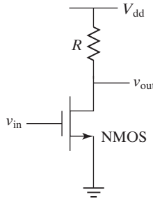
FIGURE 6–29 A simple MOSFET amplifier.
