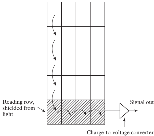
FIGURE 5–31 Architecture of a two-dimensional CCD imager. The arrows show the path of the charge-packet movement.
