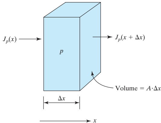
FIGURE 4-16 In steady state, the number of holes flowing into the box per second is equal to the number of holes flowing out per second plus the number of holes lost to recombination in the box per second.
