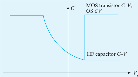
FIGURE 5-19 C-V curves of MOS capacitor and transistor.
