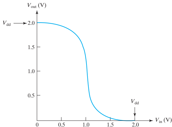
FIGURE 6-19 The VTC of a CMOS inverter.
