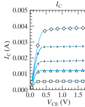
FIGURE 8-14 Ebers–Moll model (line) agrees with the measured data (symbols) in both the saturation and linear regions. I_B = 4.3, 11, 17, 28, and 43 \mu\text{A} . High-speed SiGe-base BJT. A_E = 0.25 \times 5.75 \mu\text{m}^2 . (From [3].)
