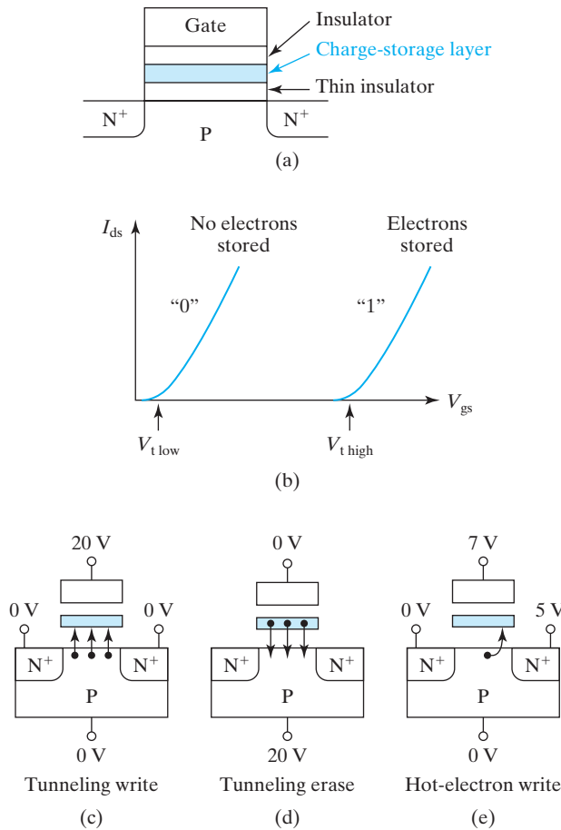
FIGURE 6-37 (a) A charge-storage NVM cell has a charge-storage layer in the gate dielectric stack; (b) V_t is modified by trapping electrons; (c) electron injection by tunneling; (d) electron removal by tunneling; and (e) electron injection by hot-electron injection.
