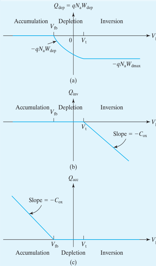
FIGURE 5-13 Components of charge ( \text{C}/\text{cm}^2 ) in the MOS capacitor substrate: (a) depletion-layer charge; (b) inversion-layer charge; and (c) accumulation-layer charge.
