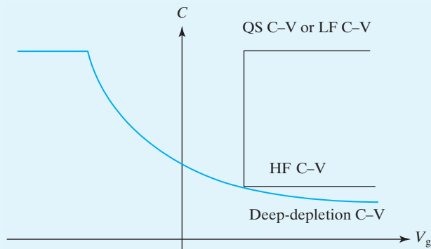
FIGURE 5-29 Deep-depletion C-V.
