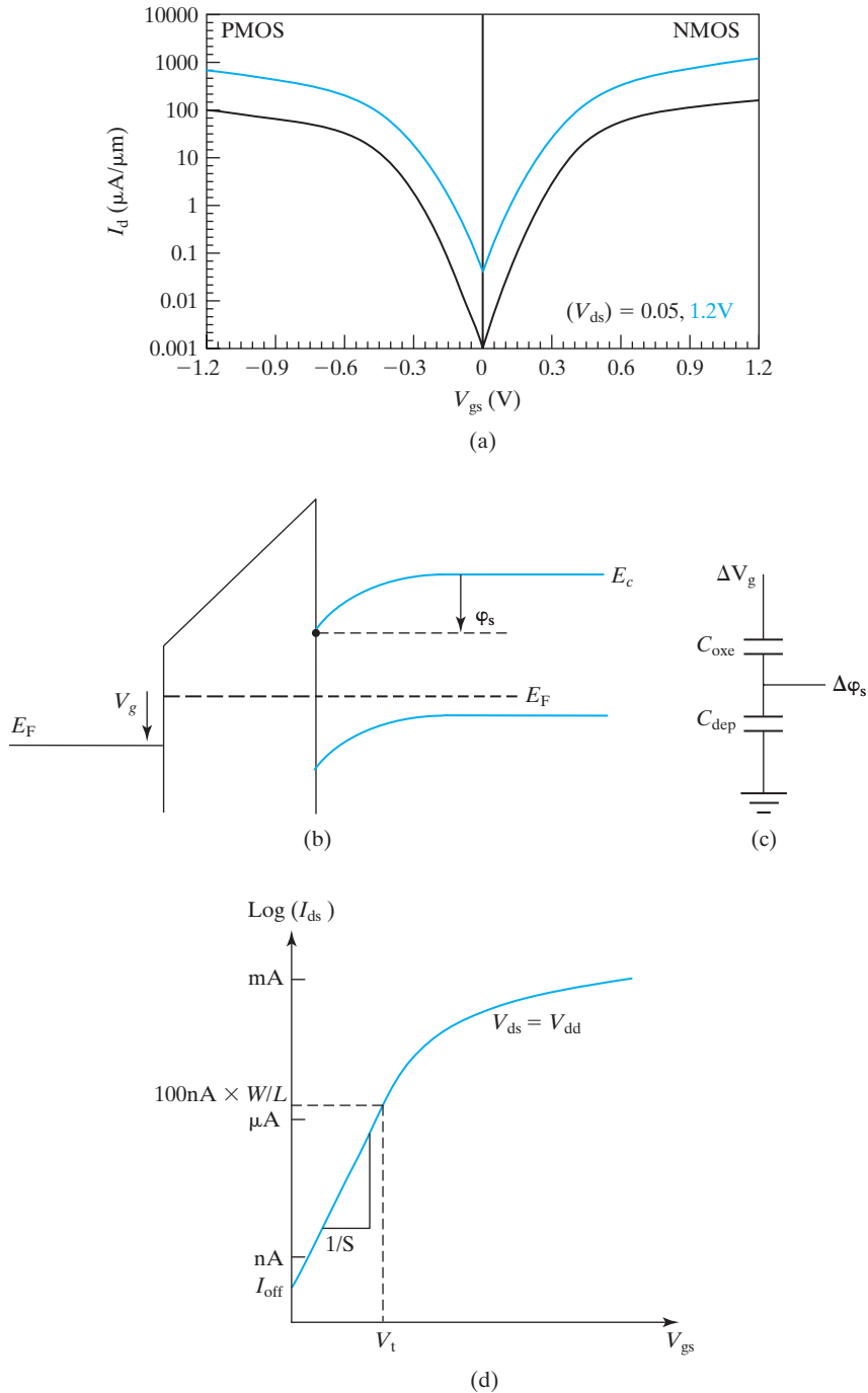
FIGURE 7-2 The current that flows at V_{gs} < V_t is called the subthreshold current. V_t \sim 0.2\text{ V} . The lower/upper curves are for V_{ds} = 50\text{ mV}/1.2\text{ V} . After Ref. [2]. (b) When V_g is increased, E_c at the surface is pulled closer to E_F , causing n_s and I_{ds} to rise; (c) equivalent capacitance network; (d) subthreshold I-V with V_t and I_{\text{off}} . Swing, S , is the inverse of the slope in the subthreshold region.
