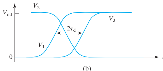
FIGURE 6-20 (a) A CMOS inverter chain. A circle on the gate indicates a PFET. (b) Propagation delay, \tau_d , defined.
