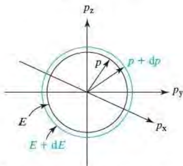
FIGURE I-2 Each sphere in the momentum space represents a constant-energy surface.
