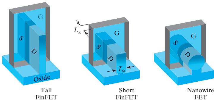
FIGURE 7–19 Variations of FinFET. Tall FinFET has the advantage of providing a large W and therefore large I_{\text{on}} while occupying a small footprint. Short FinFET has the advantage of less challenging lithography and etching. Nanowire FET gives the gate even more control over the transistor body by surrounding it. FinFETs can also be fabricated on bulk Si substrates.
