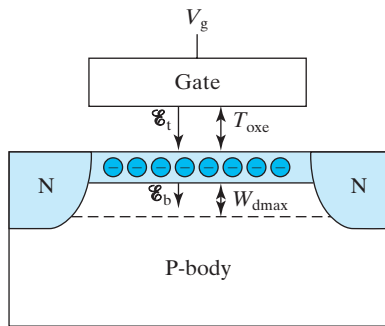
FIGURE 6–8 Surface mobility is a function of the average of the electric fields at the bottom and the top of the inversion charge layer, \mathcal{E}_b and \mathcal{E}_t .
